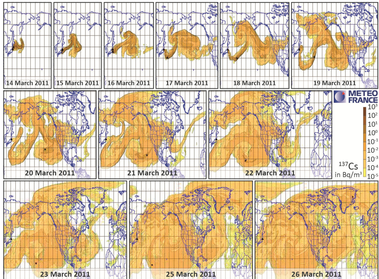
FIG. 4.1. Results from one of the global models of the atmospheric dispersion of ^{137}\text{Cs} , presented in its original code of colours (see Ref. [180] for details) (Illustration courtesy of Meteo-France).
