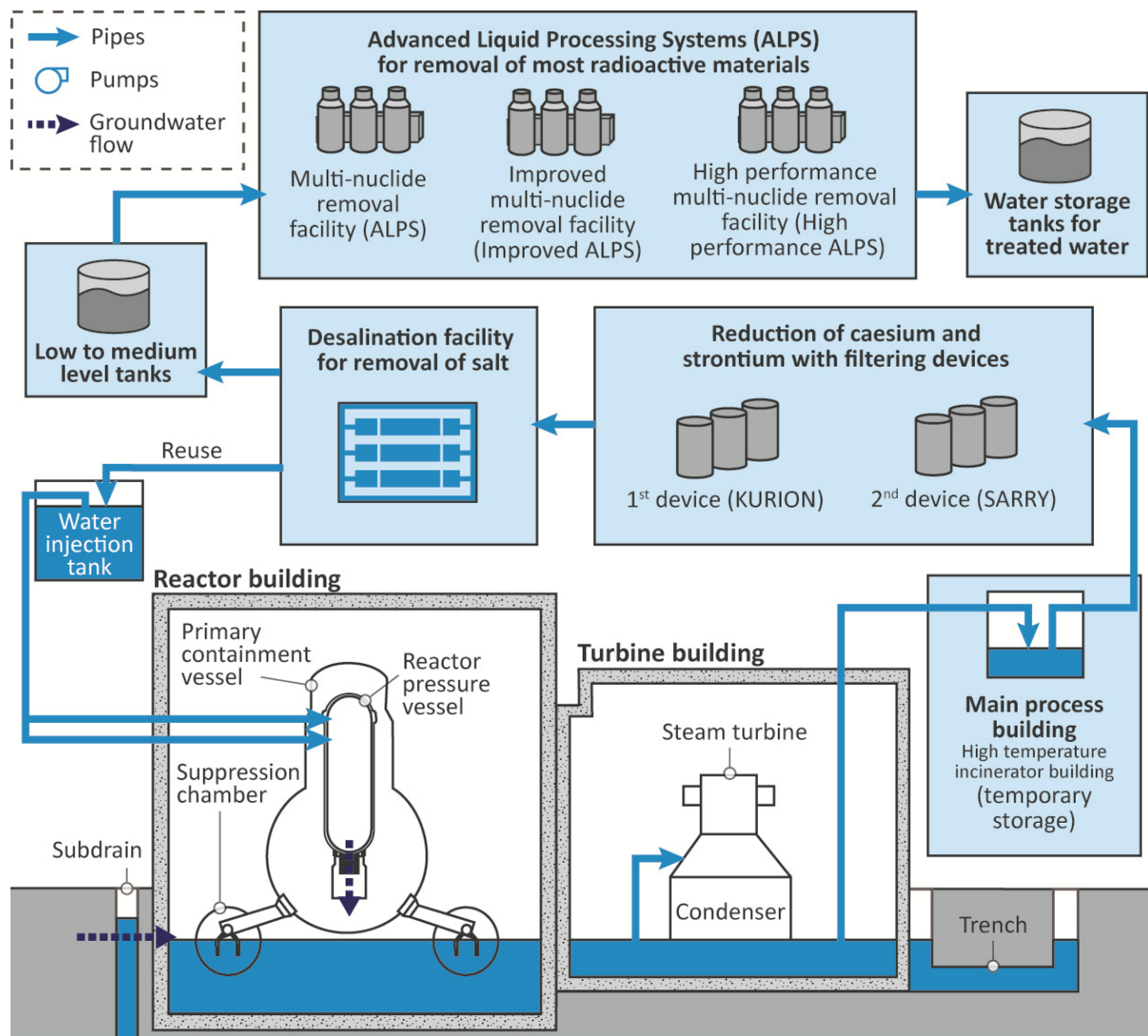
FIG. 5.4. Management of contaminated water on the site [284].
