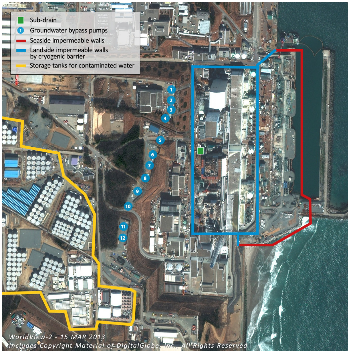
FIG. 5.5. Illustration of water management efforts. Storage tanks for contaminated water are shown on the left [286].
